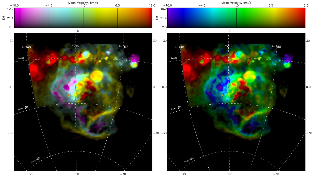
Fig. 2.— Examples of two-dimensional color images. Left panel: color represents the mean velocity of the H\alpha line in the Orion-Eridanus superbubble and is depicted with the physiologically-desirable pseudo colortable. Right panel: the same, but using a physiologically-incorrect rainbow-like colortable.
