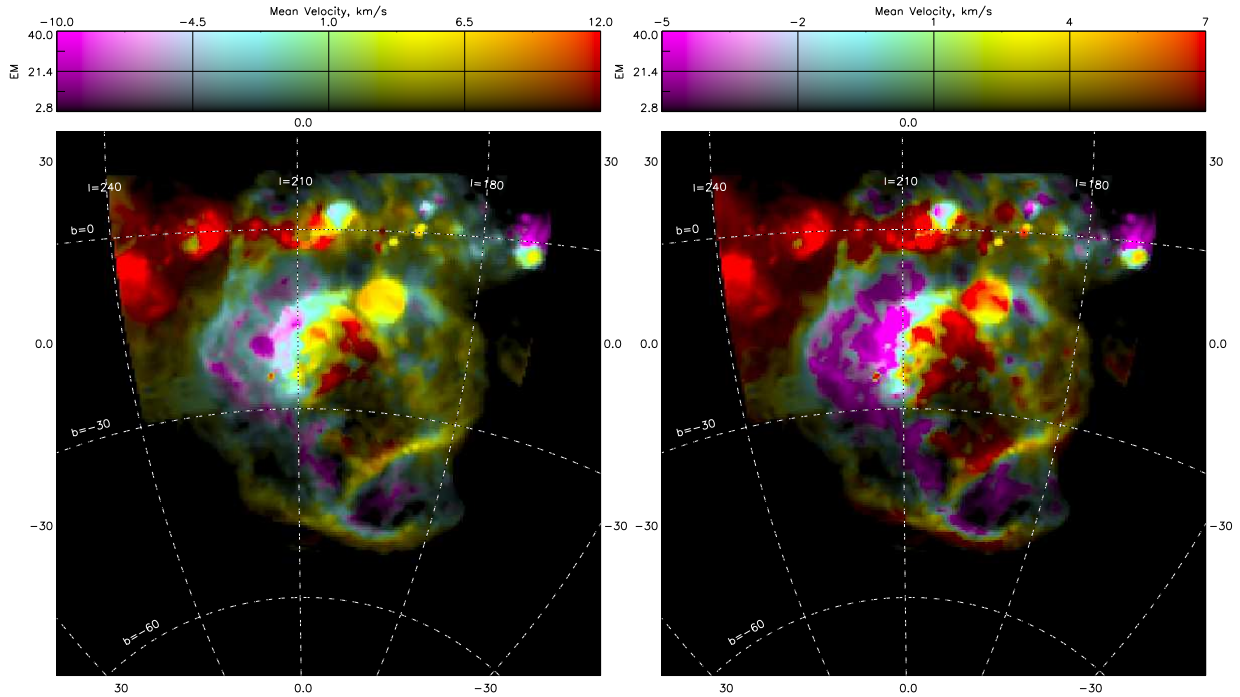
Fig. 5.— The same image as the left-hand panel of Figure 2, but with the colors spanning the smaller velocity range ( -5 to +7 ) km/s.
