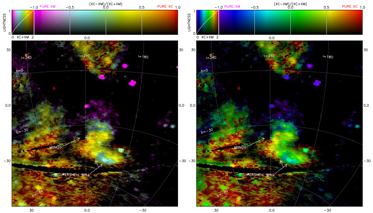
Fig. 3.— A two-dimensional color images. Left panel: color represents the X-ray energy, and thus the hot gas temperature, in the Orion-Eridanus superbubble and is depicted with the physiologically-desirable pseudo colortable. Right panel: the same, but using a physiologically-incorrect rainbow-like colortable.
