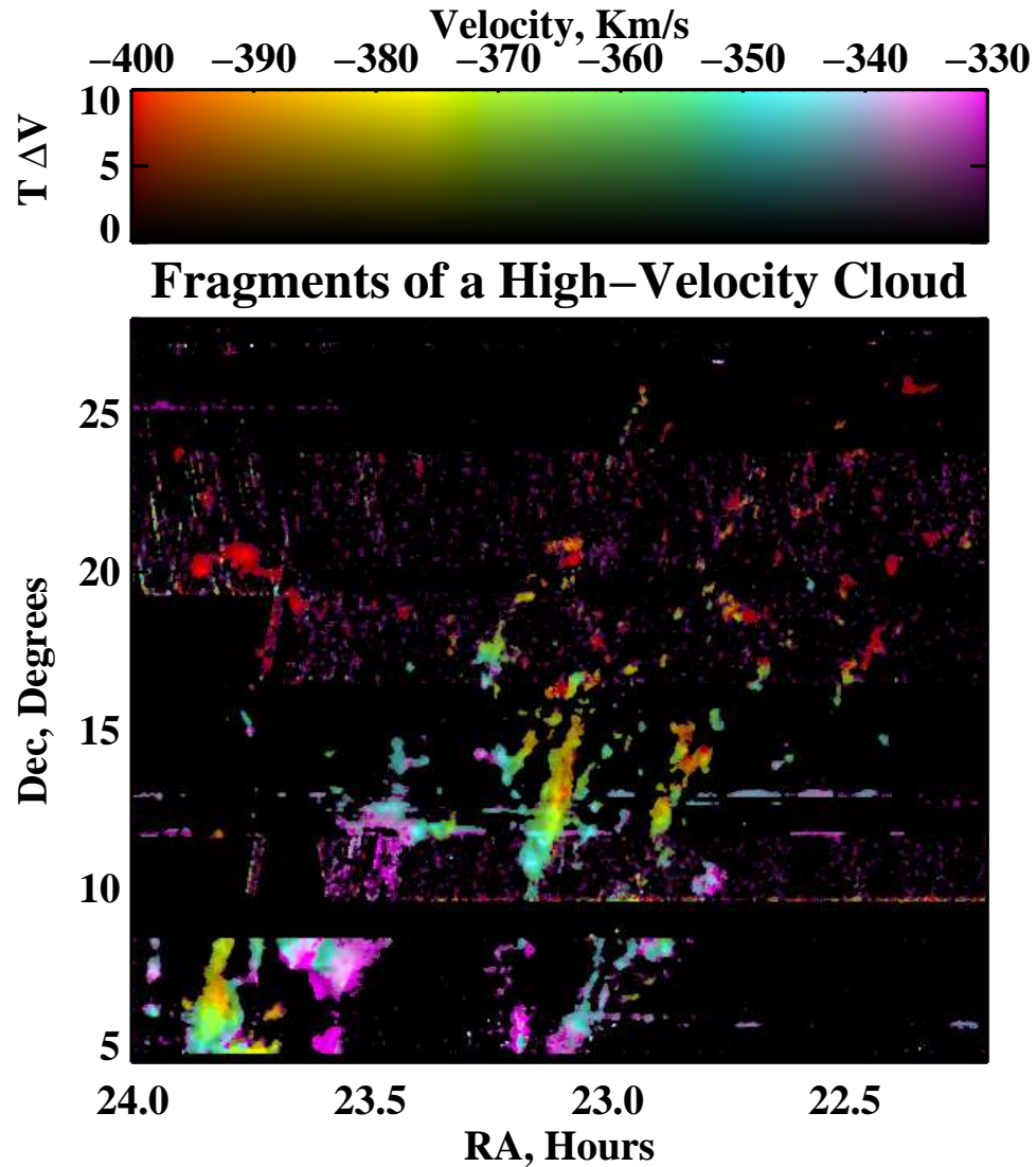
Fig. 8.— The 2-d image produced by the sample IDL code. It's high-velocity clouds.
