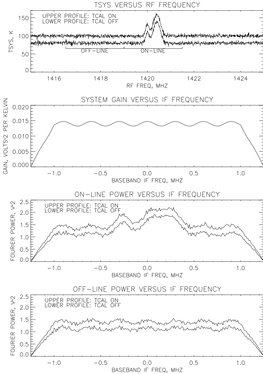
Fig. 1.— An HI line profile and its system contaminates, which must be removed by calibration.
