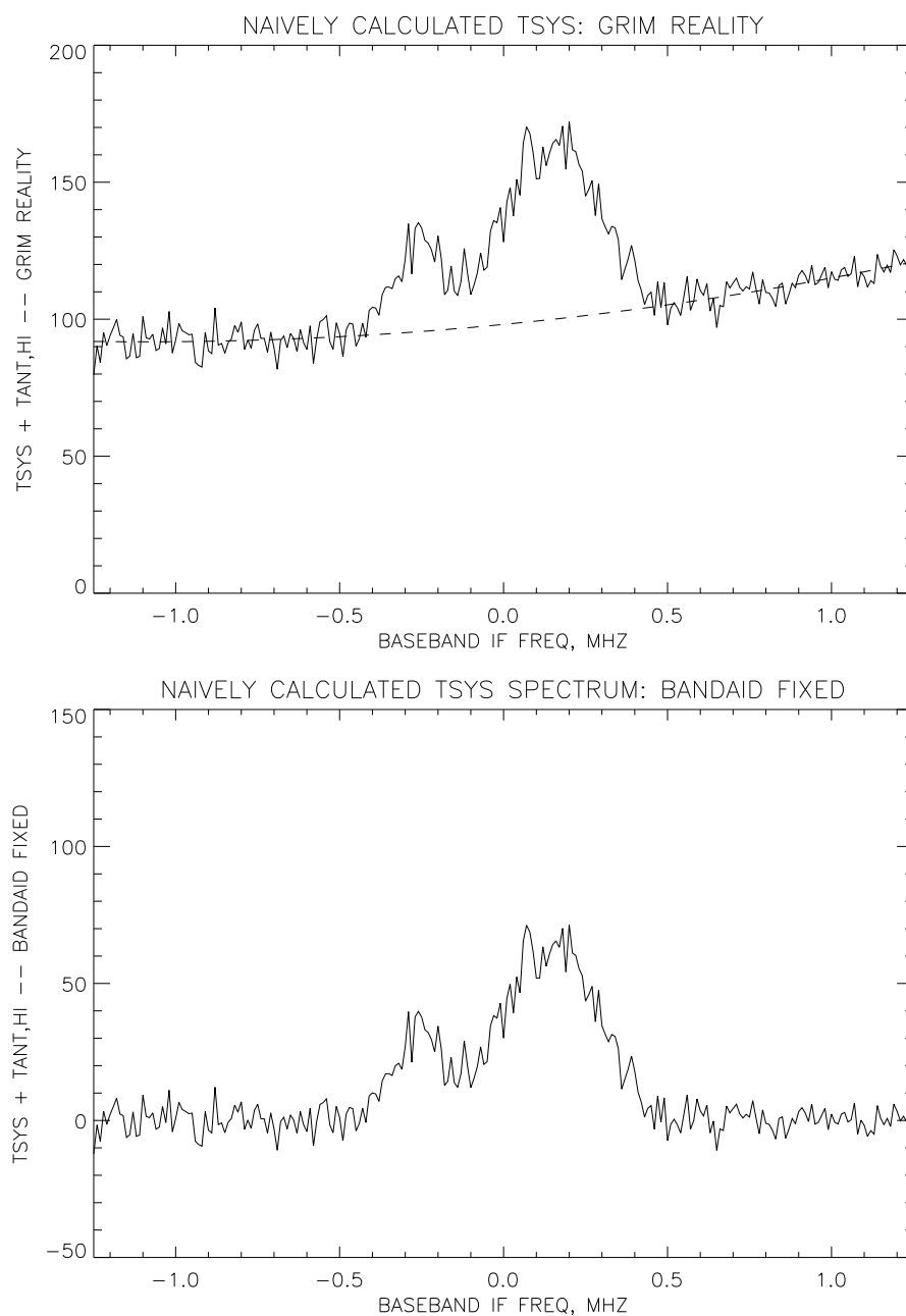
Fig. 3.— The grim reality in spectral line measurements. Departures from our ideal assumptions produce curved, displaced baselines, shown in the top panel. Fitting a polynomial baseline with least squares and subtracting it produces the apparently perfect spectrum in the bottom panel.
