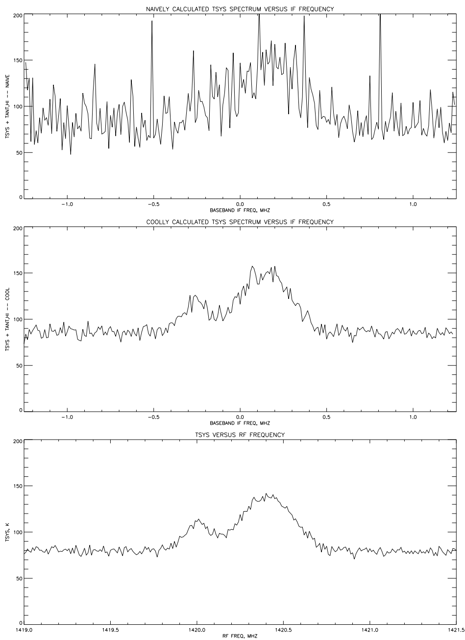
Fig. 2.— Top two panels: two different reduction techniques: naïve and cool. Bottom panel: the ON-LINE spectrum from the top panel of figure 1
